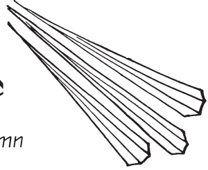
Six-sided Needles
